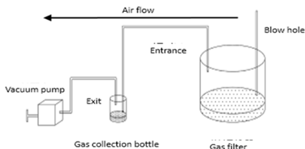
Fig. 1: Sketch of \text{NH}_3 absorption equipment in the field plots
