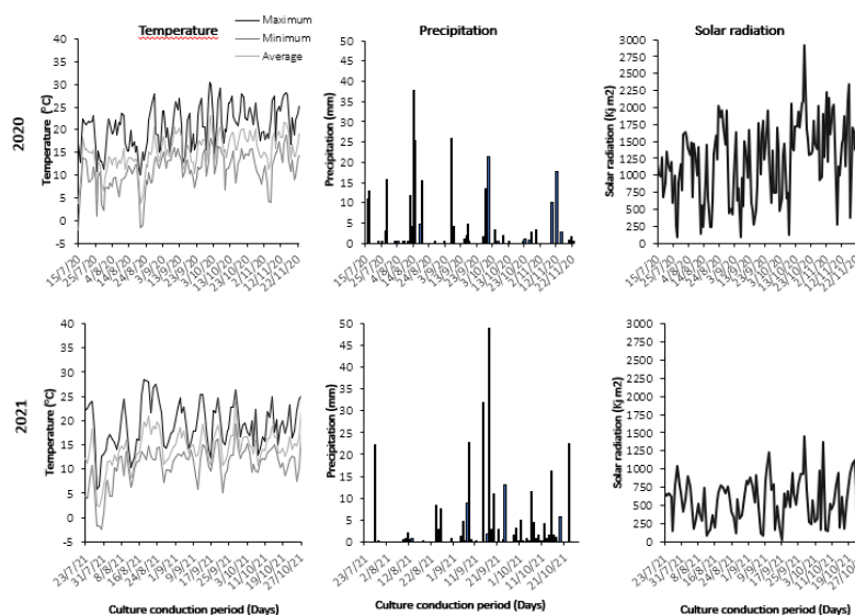
Fig. 1: Temperature maximum ( T^{\circ} \text{MAX} ), minimum ( T^{\circ} \text{MIN} ) and average ( T^{\circ} \text{MEAN} ), rainfall and global solar radiation global during experiments with artificial continuous shading on white oat. Lages-SC, 2020/20 e 2021/21 growing seasons Source: Adapted from INMET (2019)
