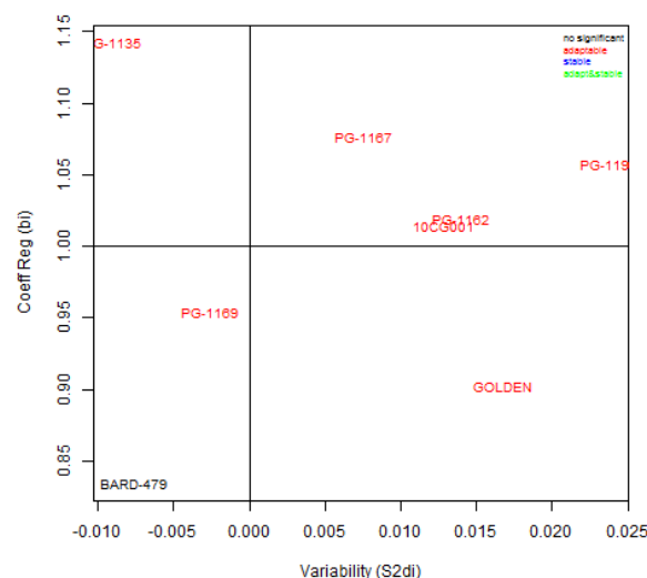
Fig. 2: Eberhart and Russel (1966) stability plot for coefficient of yield
