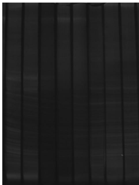
Fig. 2: Effects of different concentrations of dimethylpentylene on the diversity of soil bacterial community in the field From left to right: 0, 200, 400, 600, 800, 1000, 1200, 1400 g a.i. ha ^{-1}
