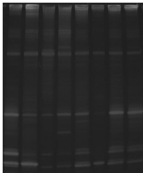
Fig. 4: Effect of different concentrations of dimethylpentylene on the diversity of soil fungal community in the field
