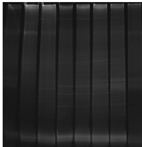
Fig. 3: Effect of different concentrations of dimethylpentylene on diversity of soil fungal community in pot
