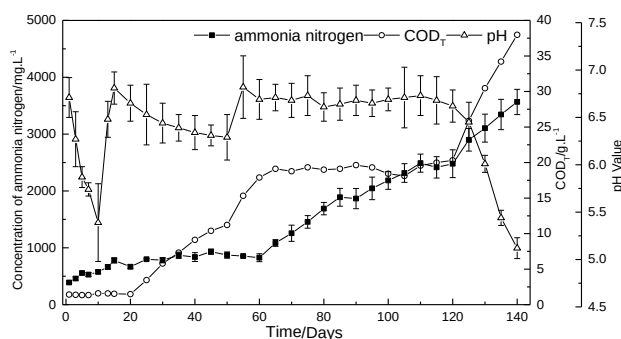
Fig. 2: The changes of pH, the ammonia nitrogen and COD T concentration in R2 reaction
