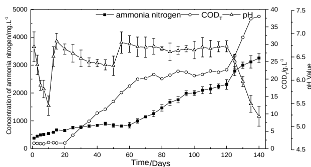
Fig. 3: The changes of pH, the ammonia nitrogen and COD T concentration in R3 reaction
