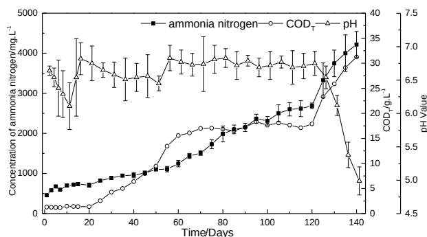
Fig. 1: The changes of pH, the ammonia nitrogen and COD T concentration in R1 reaction
