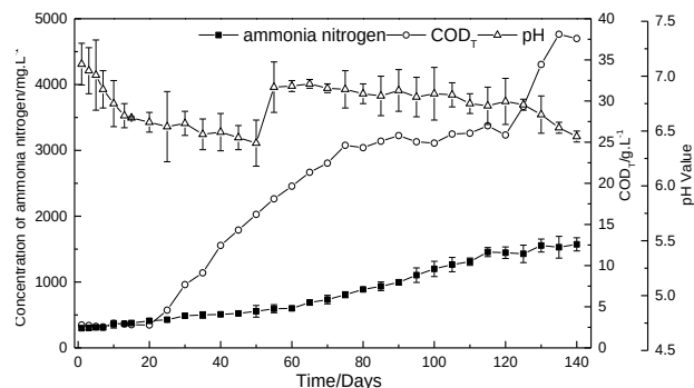
Fig. 4: The changes of pH, the ammonia nitrogen and COD T concentration in R4 reaction
